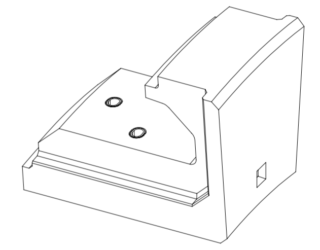
Male block, drawing 14-151-014 Fastening : 4 screw M 24 x 200, inox 304 8 washers M 24, inox 304 4 nuts M 24, inox 304
