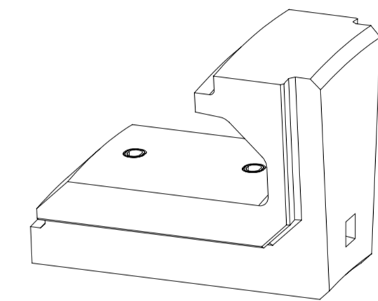
Female block, drawing 14-151-013 Fastening : 2 screw M 24 x 200, inox 304 4 washers M 24, inox 304 2 nuts M 24, inox 304
