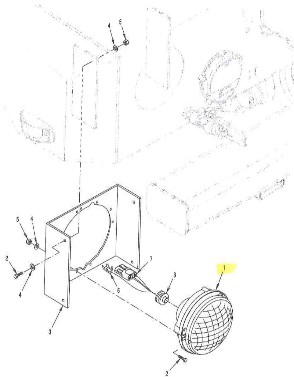
Figure 105. Headlight Assembly.
