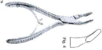
CLEVELAND 32.103.14 14 cm/5 1/2"
